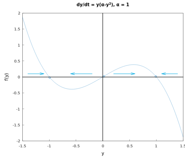
Figure 5.52: The plot for f(y) = y(\alpha - y^2) with \alpha = 1 , the phase line is drawn with the blue arrows (Hamzstplot/Examples with Makefile/Differential Equations/Plot 2D for Bifurcation Points Problem 26 2 Equilibrium Solutions/main.cpp).
